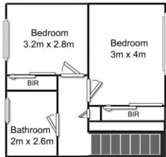
Top Floor
